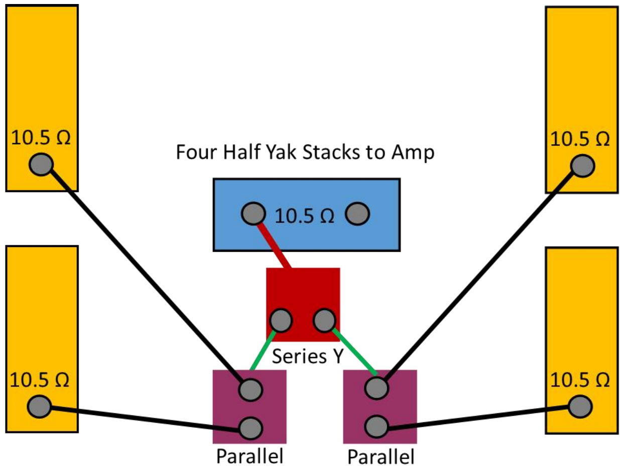
Parallel Adapter
